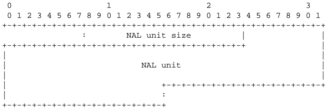
Figure 6. Structure for single-time aggregation unit
